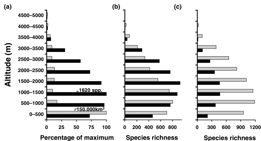
Figure 2 Species richness and number of endemics per elevational zone (500 m intervals on y-axis) in Ecuador. (a) In order to compare patterns of area size and species richness, values on x-axis were rescaled, expressing the maximum of each individual graph as 100%. This maximum is indicated for the respective maximum class. Black bars: species richness of Ecuadorian epiphytes; grey bars: area size of each elevational zone. (b) Epiphyte species richness: orchids (black bars) vs. all other taxa (grey bars). (c) Richness of epiphytes: endemics (black bars) vs. non-endemics (grey bars). Analyses based on data from Jørgensen & León-Yáñez (1999) and Valencia et al. (2001).
