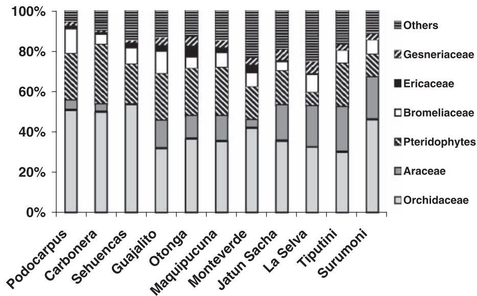
Figure 3 Proportion of families among species richness of Neotropical epiphyte inventories. All fern families summarized under 'Pteridophyta'.
