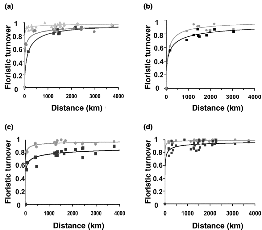
Figure 4 Floristic turnover (complement of Sørensen-Index) as a function of distance between Neotropical epiphyte inventories. Each symbol represents a pair of two compared sites. (a) Black boxes (and line): lowland vs. lowland inventories: n = 7 , r^2 = 0.72 , dark grey circles (and line): Montane vs. montane inventories ( n = 22 , r^2 = 0.79 ), hatched bright grey triangles (and uppermost line): lowland vs. montane inventories ( n = 28 , r^2 = 0.79 ). All P < 0.01 . (b–d) For the same patterns, the floristic turnover in Orchidaceae (grey lines and circles) and Pteridophyta (black lines and boxes) are compared. (b) Lowland inventories vs. lowland inventories; (c) Montane vs. montane inventories; (d) lowland vs. montane inventories. Regression lines: best fit nonlinear regressions. N as in graph A, all r^2 > 0.64 , all P < 0.01 .
